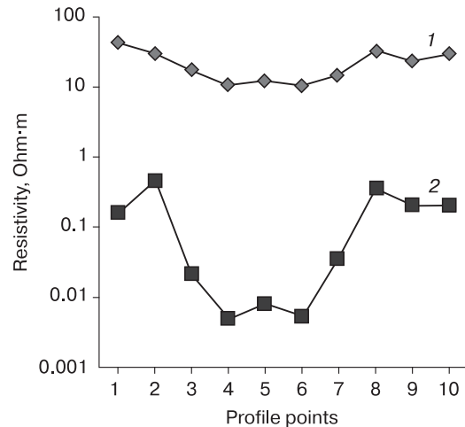
Fig. 2. Variations of apparent resistivity (1) and electromagnetic resistivity (2) at 549 kHz along a profile that traverses a supra-permafrost talik.
