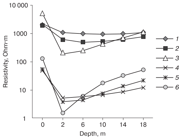
Fig. 1. Calculated dependence of apparent resistivity (lines 1–3) and electromagnetic resistivity (lines 4–6) on depth of conducting unfrozen water-bearing porous fine-grained zones in permafrost.
