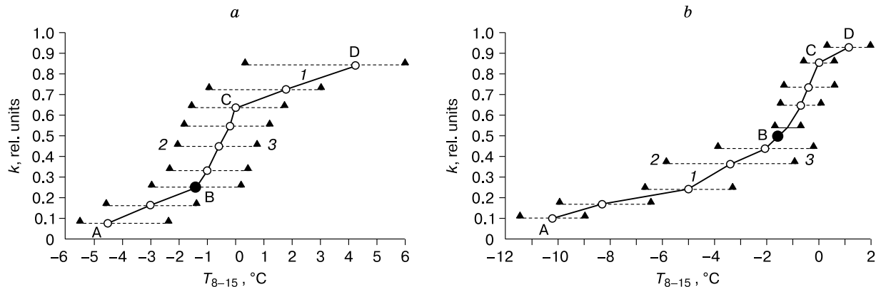
Fig. 3. Correlation of average median values of attenuation k of GPR ( a ) and induction ( b ) responses with temperature in active layer at a depth of 8–15 m: specific aggregated regional models.
