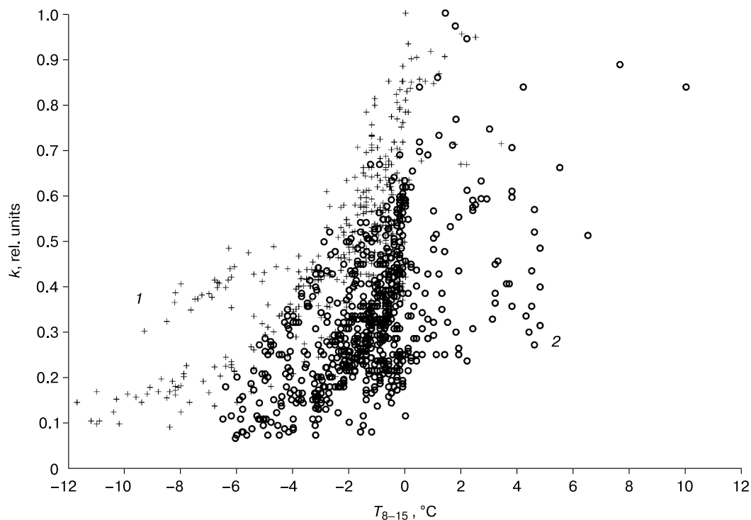
Fig. 2. Correlation of normalized attenuation ( k ) of induction (curve 1) and GPR (curve 2) responses with temperature in active layer at a depth of 8–15 m ( T_{8-15} , °C): a general regional model.
